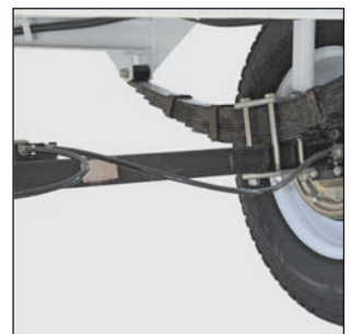
Braking system with Gabriel shock absorbers
